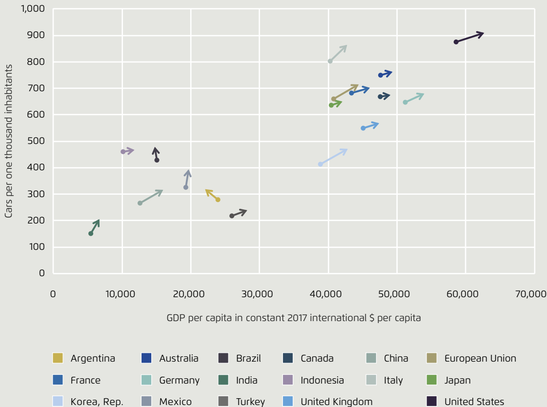
Development of per capita GDP and vehicle ownership in selected G20 countries 2015–2019 Figure 2.7
