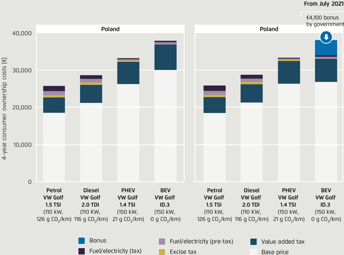
4-year consumer ownership costs for comparable passenger cars in Poland by fuel type in 2020 (left) and 2021 (right)
